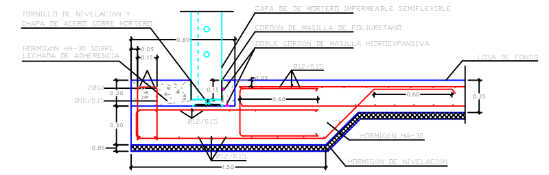
DETALLE 1 E: 1/40
