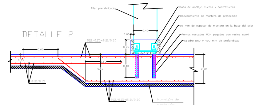
DETALLE 2 E: 1/40
